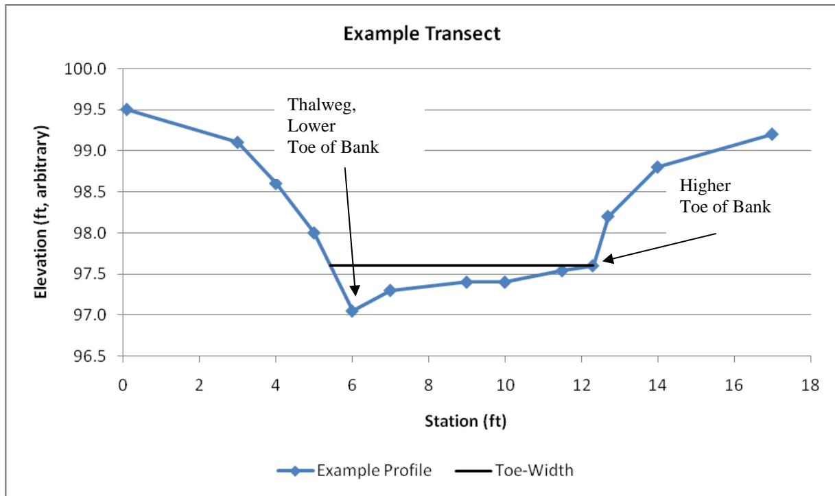
Figure 2. Example of Thalweg and Toe of Bank Coinciding
