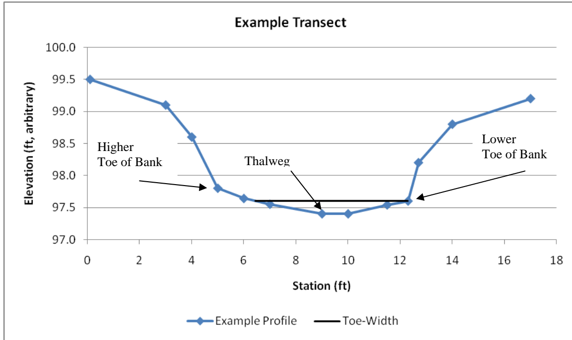
Figure 1. Example of Toe-Width Interpolation
